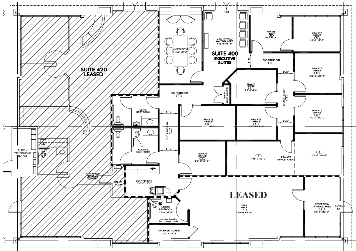
Floor Plan
